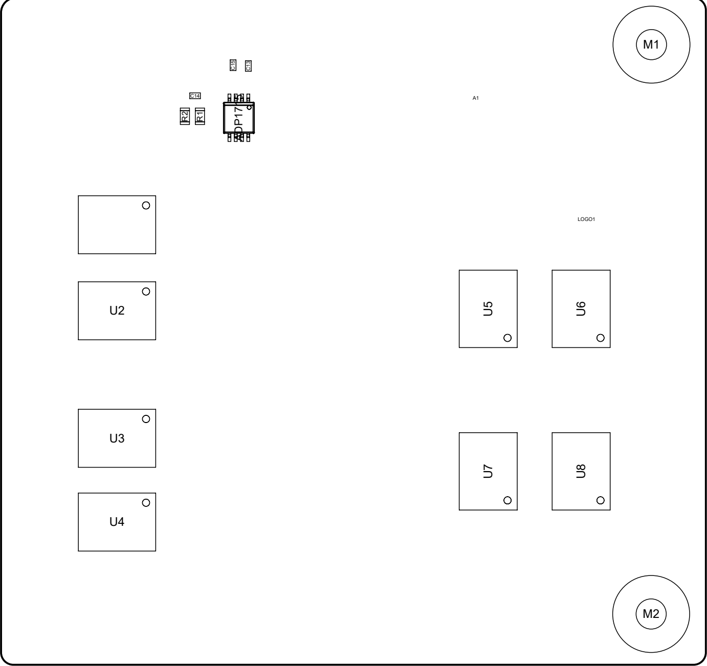
View from Top side (Scale 5:2)
